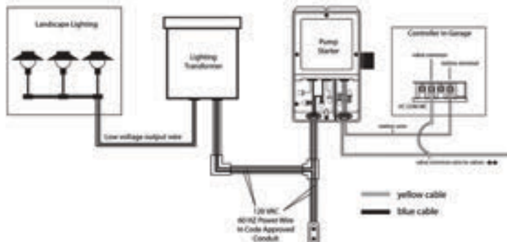
SR-1 AS A LANDSCAPE LIGHTING RELAY
